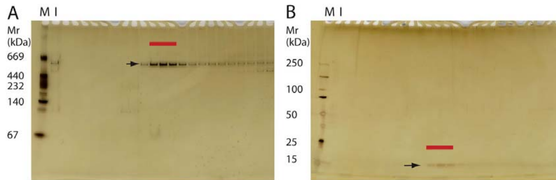
Figure S9. Purification of riboflavin synthase. Fractions from the HIC column were analyzed by native PAGE (A) and SDS PAGE (B). Black arrow in A shows the riboflavin synthase and in B shows riboflavin synthase \beta subunit (DVU1198). \alpha subunit (DVU1200) couldn't be seen on PAGE and was identified by MS/MS. Red bars show the fraction used for EM analysis. Molecular weight standards are shown in lane M. The input fraction to the HIC column is shown in lane I.
