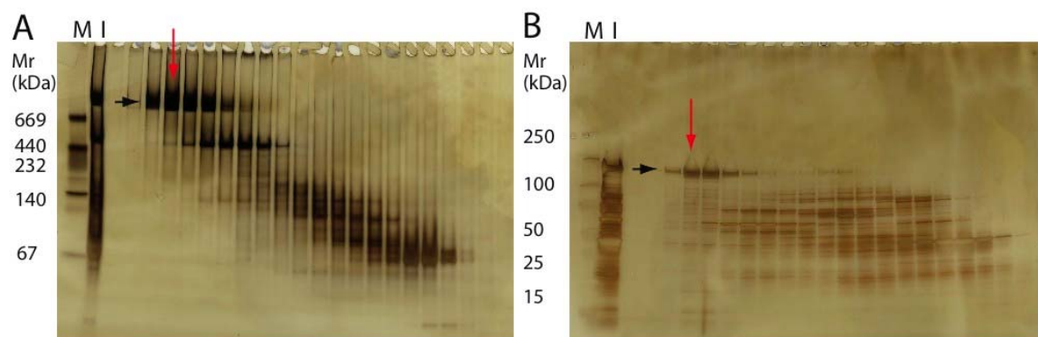
Figure S17. Purification of PFOR. Fractions of the SEC column were analyzed by native PAGE (A) and SDS PAGE (B). Black arrows show the PFOR. Red arrows show the fraction used for EM analysis. Molecular weight standards are shown in lane M. The input fraction to the SEC column is shown in lane I.
