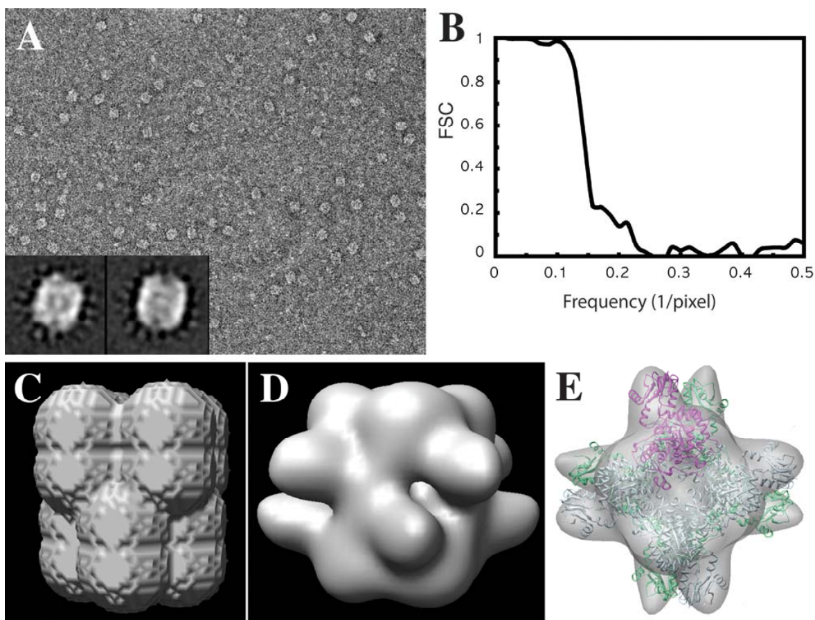
Figure S34. IMP dehydrogenase EM data, refinement result, and docking of a pseudo-atomic model structure. 5814 particles were used for the refinement C4 symmetry was imposed during the refinement. The standard FSC curve falls to 0.5 at a resolution of 19 Å after two rounds of refinement, each of which consisted of 15 cycles. (a) Electron micrograph of the negatively stained IMP dehydrogenase sample. Two examples of class averages are shown at the bottom left. (b) Fourier shell correlation curve. (c) An intuitive starting model was built from 16 partially overlapping spheres in a way that reflected the number of subunits expected from the estimated particle weight (and the known molecular weight of the protein monomer) and some of the views seen in the class averages. (d) A side view of the refined structure. (e) A top view in which a homology model, built from a PDB template 1ZFJ, was docked into the semitransparent EM density. Tetramer at the bottom is shown as light green ribbons and the one at the top as light blue ribbons with a monomer shown as magenta ribbon.
