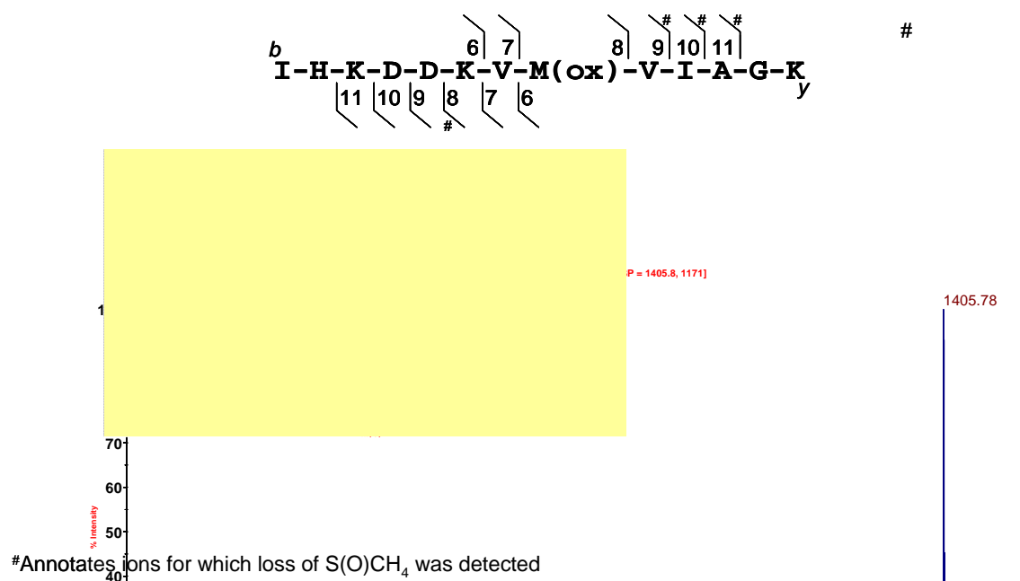
Figure S25: Identification of 50S ribosomal protein L24 (DVU1314, Q72CG9, gene rplX) by MS/MS analysis of molecular m/z 1469.76: IHKDDKVM(ox)VIAGK.
