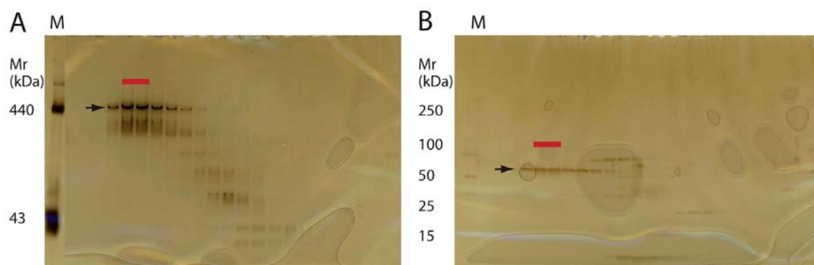
Figure S6. Purification of putative protein (DVU0671). Fractions of the SEC column were analyzed by native PAGE (A) and SDS PAGE (B). Black arrows show the putative protein. Red bars show the fraction used for EM analysis. Molecular weight standards are shown in lane M.
