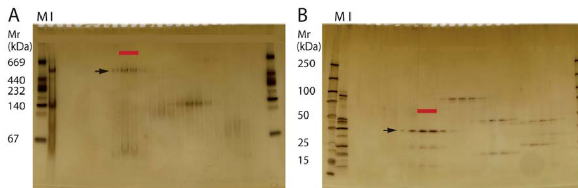
Figure S10. Purification of ketol-acid reductoisomerase. Fractions of the SEC column were analyzed by native PAGE (A) and SDS PAGE (B). Black arrows show the ketol-acid reductoisomerase. Red bars show the fraction used for EM analysis. Molecular weight standards are shown in lane M. The input fraction to the SEC column is shown in lane I.
