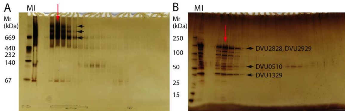
Figure S11. Purification of DNA-directed RNA polymerase. Fractions of the SEC column were analyzed by native PAGE (A) and SDS PAGE (B). Black arrows in A show DNA-directed RNA polymerase and in B show the subunits of DNA-directed RNA polymerase. \beta : DVU2928; \beta' : DVU2929; \alpha : DVU1329. \omega subunit was detected by MS but can't be seen in the gel. \sigma was not detected by MS. NusA (DVU0510) was co-purified with DNA-directed RNA polymerase. Red arrows show the fraction used for EM analysis. Molecular weight standards are shown in lane M. The input fraction to the SEC column is shown in lane I.
