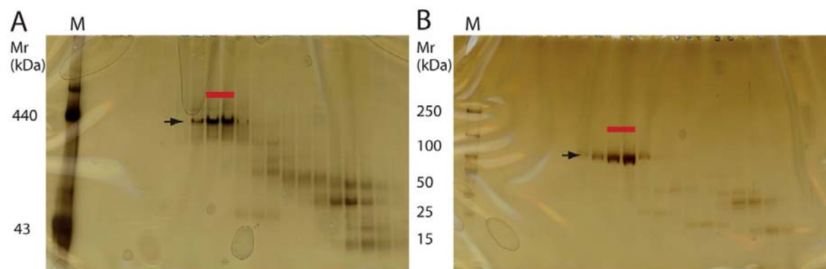
Figure S18. Purification of proline dehydrogenase/delta-1-pyrroline-5-carboxylate dehydrogenase. Fractions of the SEC column were analyzed by native PAGE (A) and SDS PAGE (B). Black arrow shows the proline dehydrogenase/delta-1-pyrroline-5-carboxylate dehydrogenase. Red bars show the fraction used for EM analysis. Molecular weight standards are shown in lane M.
