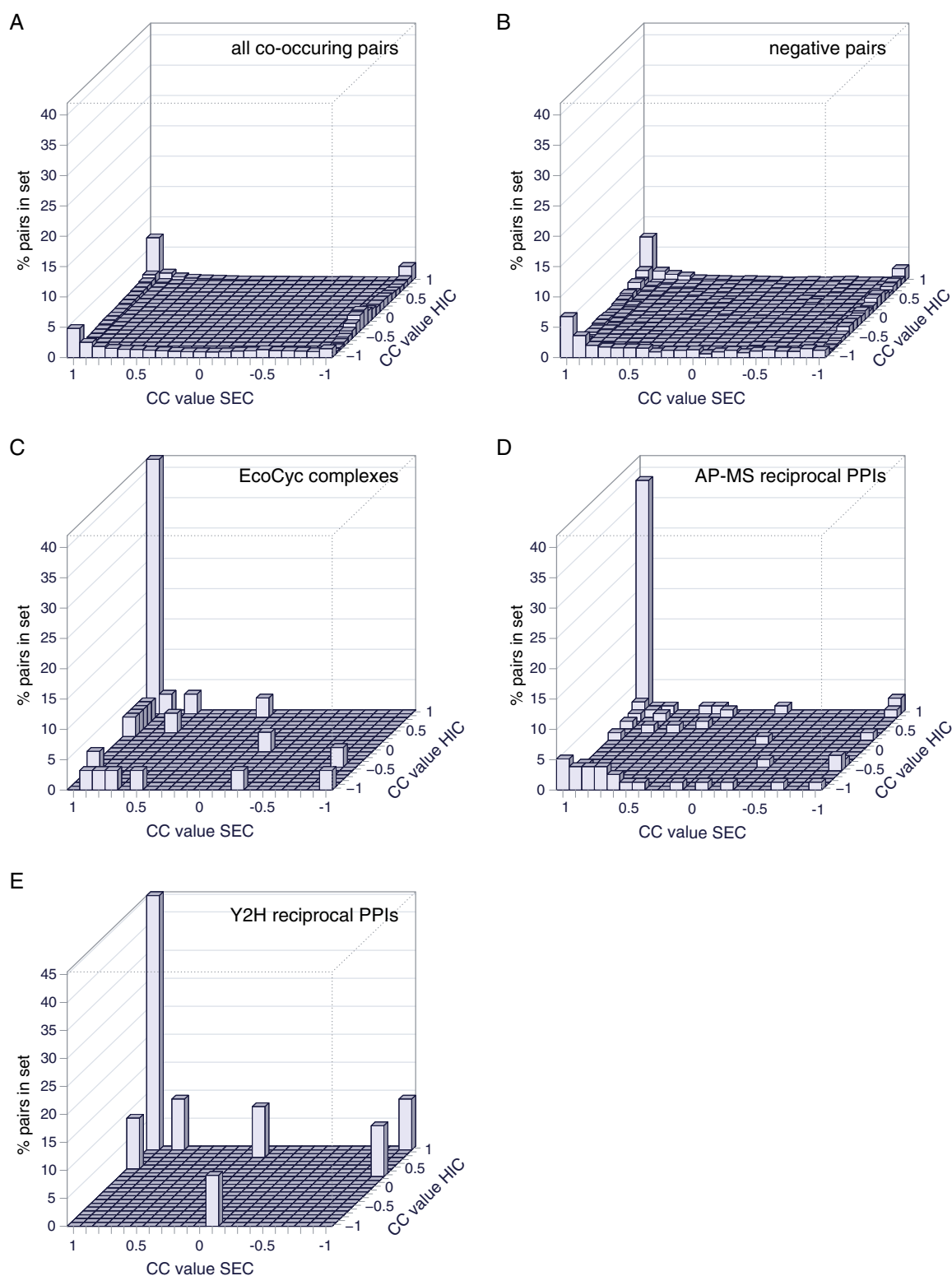
FIG. 3. Distribution of the Pearson cross correlation (CC) scores for the SEC and the HIC dimensions. Each plot shows the percentage of protein pairs in a given set that have the indicated maximum CC values for the SEC and the HIC dimensions. The two rows at -1 show the CC values where protein pairs are only detected in one dimension only. A , The set of all 146,792 co-occurring protein pairs. B , 1496 negative protein pairs unlikely to interact. C , 31 EcoCyc complex PPIs. D , 28 reciprocally confirmed AP-MS PPIs. E , 11 reciprocally confirmed Y2H PPIs. D–E are largely interologs of protein pairs defined using data from other species, except that some of the reciprocally confirmed AP-MS PPIs in D are from our D. vulgaris AP-MS interactome.
